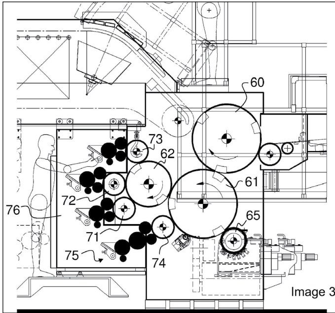
Image 3 – A schematic partial side view of a known intaglio printing press for the single-sided printing of sheets as used for the production of security documents – From Jacques P. et al (2013) – Image used in accordance with US Patent Policy – Plate Cylinder 61 and Impression Cylinder 60 with 3 segments (Image Source: Jacques P. et al – Used in accordance with the permissions granted by US Patent Office)
